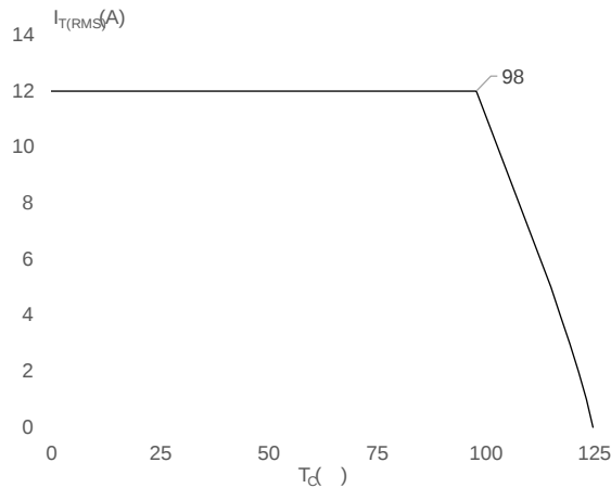
FIG.4: On-state character
