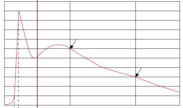
FIG.4: ESD clamping
