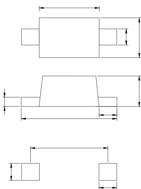
Land Pattern
