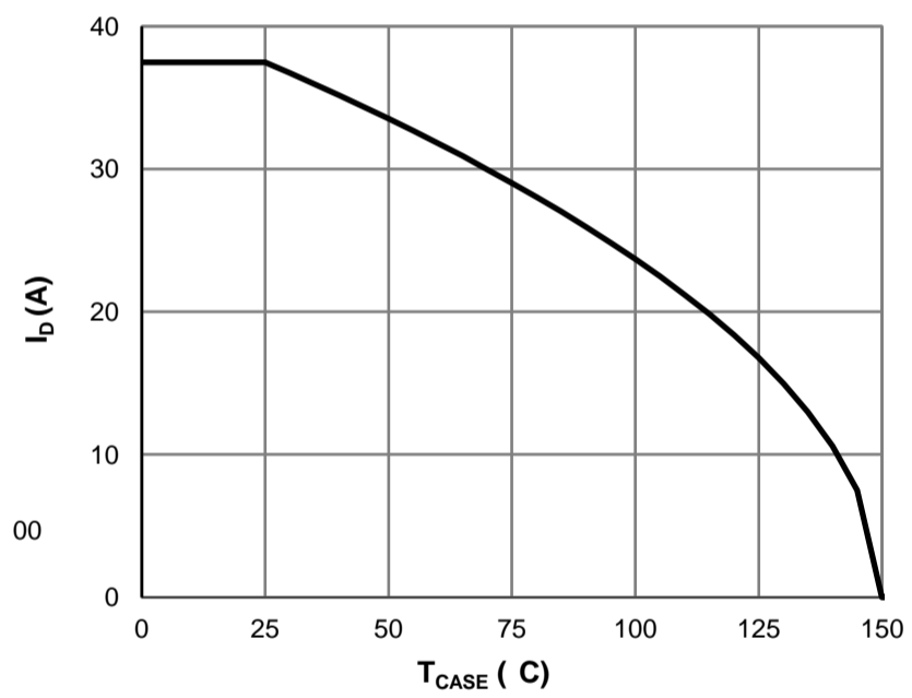
Figure 9: Current De-rating
